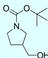
1-Boc-3-hydroxymethylpyrrolidine
