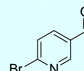
6-Bromo-3-pyridinecarboxaldehyde
