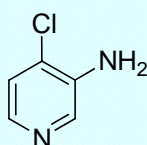
3-Amino-4-chloropyridine
