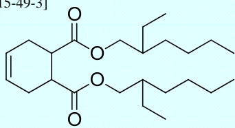
Bis(2-ethylhexyl)4-cyclohexene-1,2-dicarboxylate
