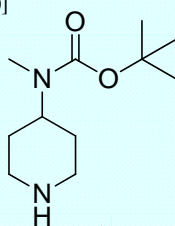
4-Boc-4-methylaminopiperidine
