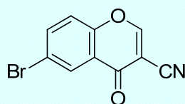
6-Bromo-3-cyanochromone
