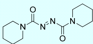
1,1'-(Azodicarbonyl)dipiperidine
