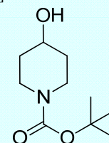
1-Boc-4-hydroxypiperidine
