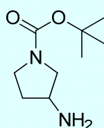
3-Amino-1-Boc-pyrrolidine
